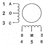
Wiring Diagram
